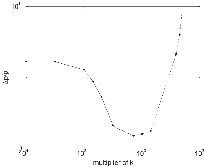
Fig. 3. The relative height of the response peak \Delta p/p with respect to the quantity that multiplies k , mimicking the stress. The dotted line indicates that the system does not display oscillatory behaviour.
