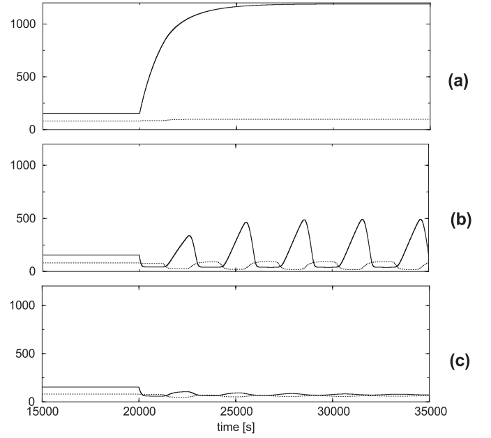
Fig. 2. The response in the concentration of p53 (solid line) and mdm2 (dotted line) upon variation of the dissociation constant k . At time 20 000 s the constant k is multiplied by 15 (a), divided by 15 (b) and divided by 5 (c).
