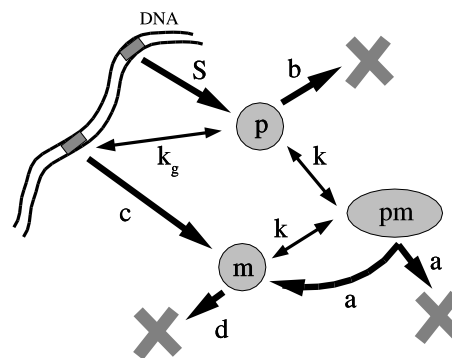
Fig. 1. A sketch of the loopback mechanism which control the amount of p53 in the cell. The grey crosses indicate that the associated molecule leaves the system.
