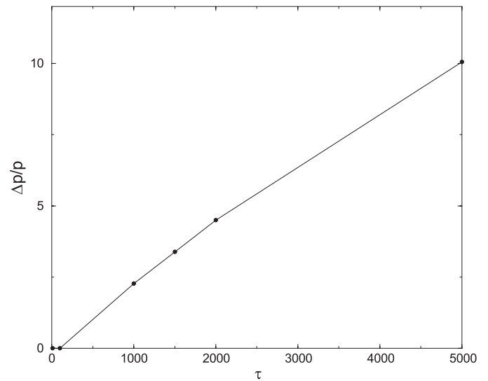
Fig. 4. The dependence of the relative height of the response peak \Delta p/p on the delay \tau .
